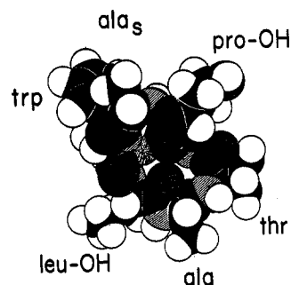
Figure 11. The conformation of phalloidin. Angles: all \omega = 0^\circ ; (\varphi, \psi)_{\text{Ala5}} = 100^\circ, 120^\circ ; (\varphi, \psi)_{\text{Trp}} = 60^\circ, 120^\circ ; (\varphi, \psi)_{\text{Leu(OH)}} = 110^\circ, 0^\circ ; (\varphi, \psi)_{\text{Ala}} = 100^\circ, 330^\circ ; (\varphi, \psi)_{\text{Thr(OH)}} = 270^\circ, 30^\circ ; (\varphi, \psi)_{\text{Cys}} = 100^\circ, 300^\circ ; (\varphi, \psi)_{\text{Hyp}} = 122^\circ, 125^\circ .
