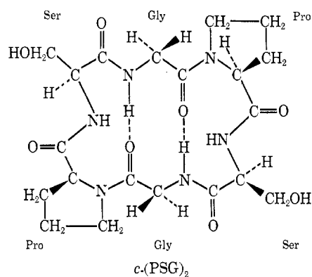
Figure 1. Spectrum (220 MHz) of cyclo -(Pro-Ser-Gly-Pro-Ser-Gly) in D_2O and (upper left) in H_2O-CH_3COOH , 98:2 (v/v); 22^\circ . The H_2O solution is made acidic to retard exchange of NH protons with solvent (see ref 40).
