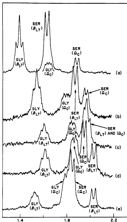
Figure 6. The 220-MHz nmr spectrum of the NH protons of cyclo -(Ser-Pro-Gly-Ser-Pro-Gly): (a) in H 2 O-CH 3 COOH, 98:2 (v/v); (b, c, and d) in DMSO- d 6 : H 2 O-CH 3 COOH (98:2); (e) in DMSO- d 6 . In (a) through (e), the mole fraction of DMSO- d 6 is 0.0, 0.5, 0.7, 0.8, and 1.0. Each spectrum is the result of 15-30 accumulated CAT scans (see ref 52).
