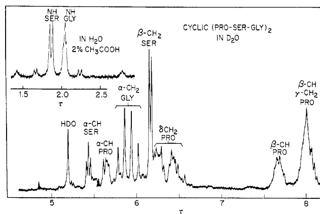
Figure 1. Spectrum (220 MHz) of cyclo -(Pro-Ser-Gly-Pro-Ser-Gly) in D_2O and (upper left) in H_2O-CH_3COOH , 98:2 (v/v); 22^\circ . The H_2O solution is made acidic to retard exchange of NH protons with solvent (see ref 40).
