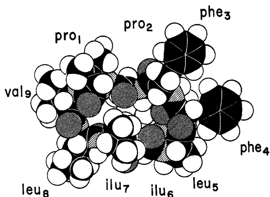
Figure 10. The conformation of cyclolinopeptide A. Angles: all \omega = 0^\circ ; (\varphi, \psi)_{\text{Pro1}} = 102^\circ, 310^\circ ; (\varphi, \psi)_{\text{Pro2}} = 122^\circ, 125^\circ ; (\varphi, \psi)_{\text{Phe3}} = 90^\circ, 330^\circ ; (\varphi, \psi)_{\text{Phe4}} = 100^\circ, 270^\circ ; (\varphi, \psi)_{\text{Leu5}} = 90^\circ, 0^\circ ; (\varphi, \psi)_{\text{Ile6}} = 90^\circ, 120^\circ ; (\varphi, \psi)_{\text{Ile7}} = 90^\circ, 120^\circ ; (\varphi, \psi)_{\text{Leu8}} = 90^\circ, 330^\circ ; (\varphi, \psi)_{\text{Val9}} = 100^\circ, 310^\circ .
