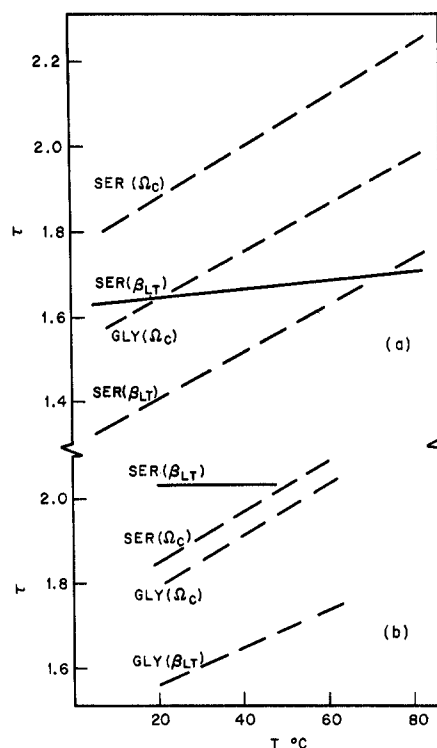
Figure 7. The temperature dependence of the chemical shifts of the NH resonances of cyclo -(Ser-Pro-Gly-Ser-Pro-Gly) in (a) H 2 O-CH 3 COOH, 98:2 (v/v); (b) in DMSO- d 6 (see ref 52).
